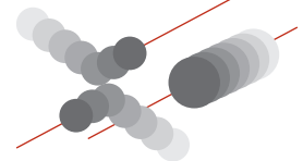
third particle interferes: no collision
