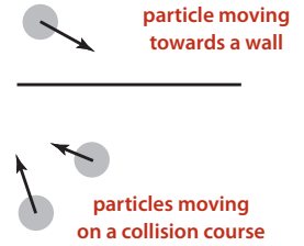
Predictable events
