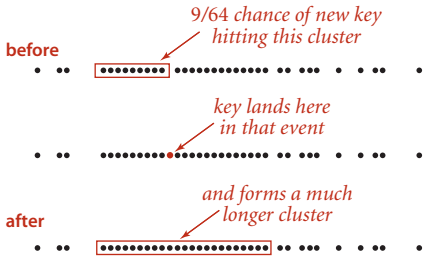
Clustering in linear probing ( M = 64 )
