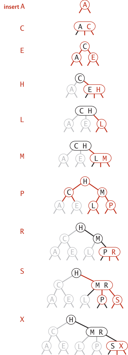
same keys in increasing order
