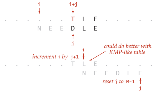
Mismatched character heuristic (mismatch not in pattern)
