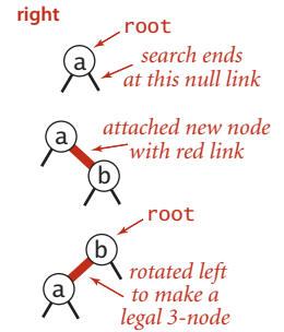
Insert into a single 2-node (two cases)
