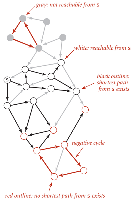
Shortest-paths possibilities
