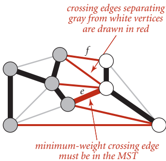
Cut property
