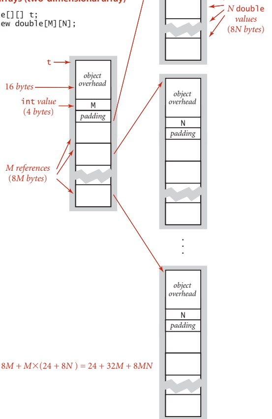
Typical memory requirements for arrays of int values, double values, objects, and arrays
