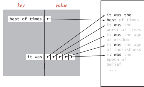
Idealized view of a text-string index
