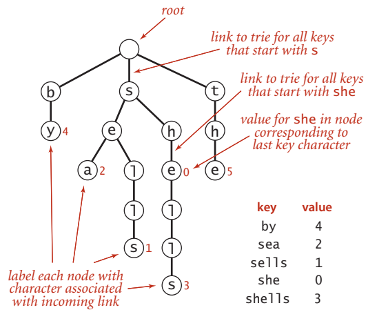
Anatomy of a trie
