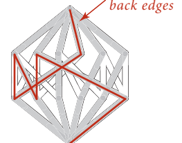
Augmenting paths for bipartite matching
