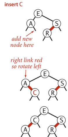
Insert into a 2-node at the bottom
